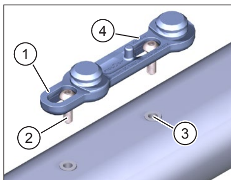
Fig. 1: Fasten the FIDLOCK® Bike Base to the e-bike
