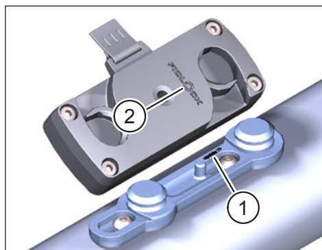
Fig. 2: Orientation of FIDLOCK® Bike Base and FIDLOCK® Force Connector
